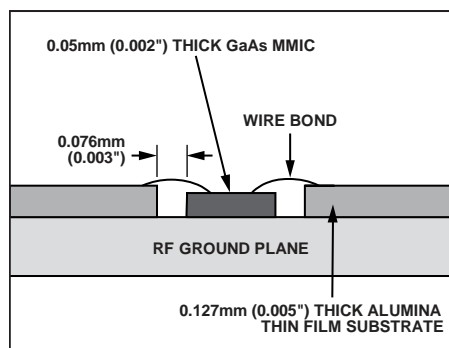
Figure 35. Routing RF Signals
