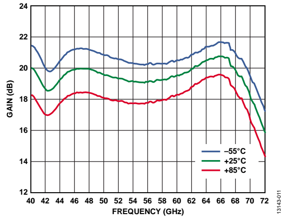
Figure 13. Gain vs. Frequency at Various Temperatures
