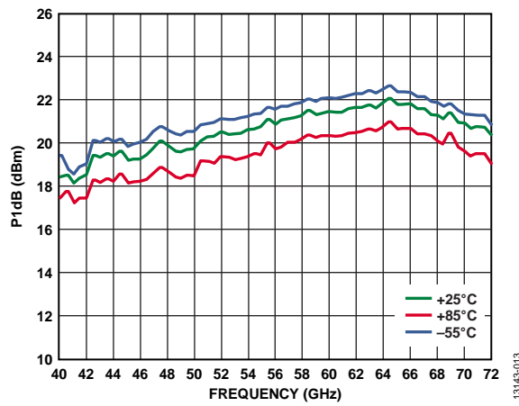
Figure 15. P 1dB vs. Frequency at Various Temperatures
