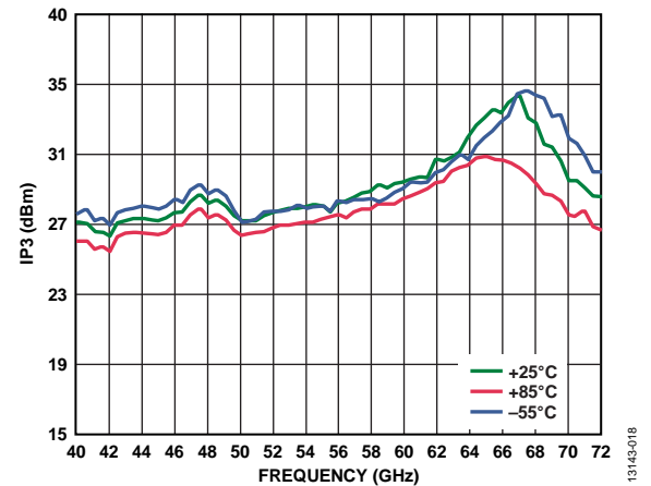
Figure 20. Output IP3 vs. Frequency for Various Temperatures at P_{OUT} = 10 \text{ dBm/Tone}
