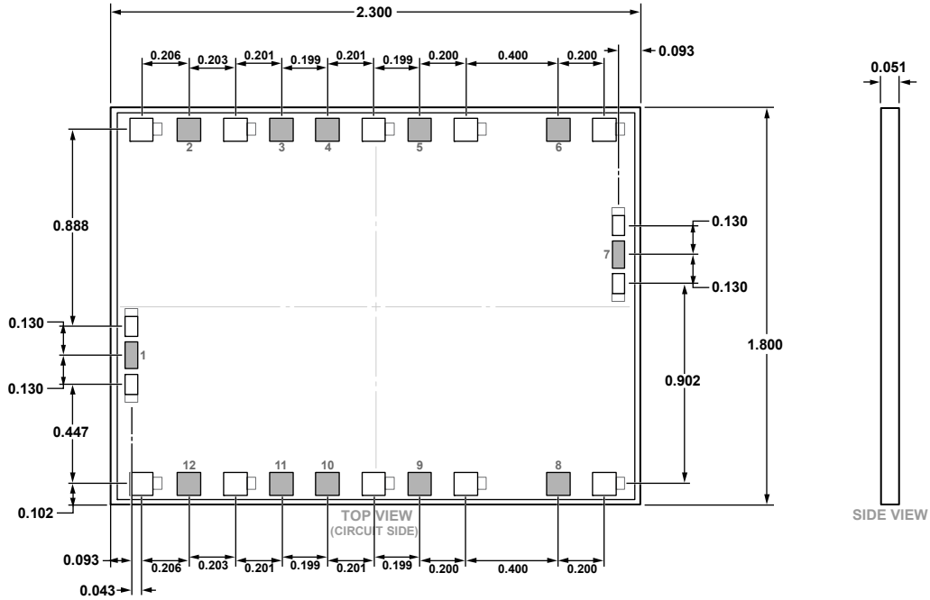
Figure 40. 12-Pad Bare Die [CHIP] (C-12-2) Dimensions shown in millimeter
