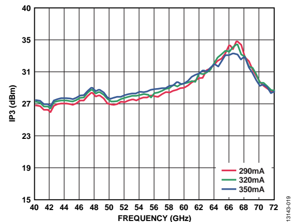
Figure 21. Output IP3 vs. Frequency for Various Supply Currents at P_{OUT} = 10 \text{ dBm/Tone}
