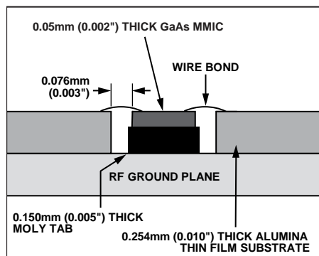
Figure 36. Routing RF Signals Using Moly Tab
