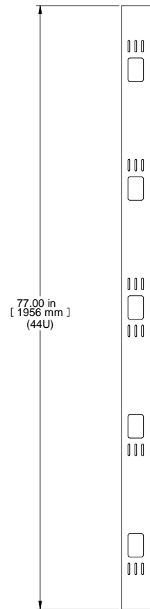
FRONT VIEW
