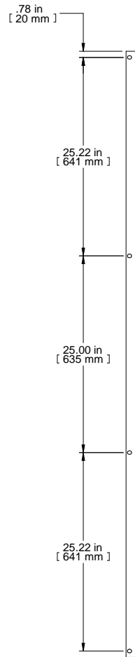
SIDE VIEW
