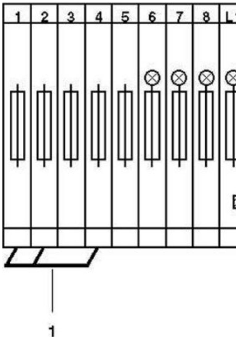
Circuit diagram
